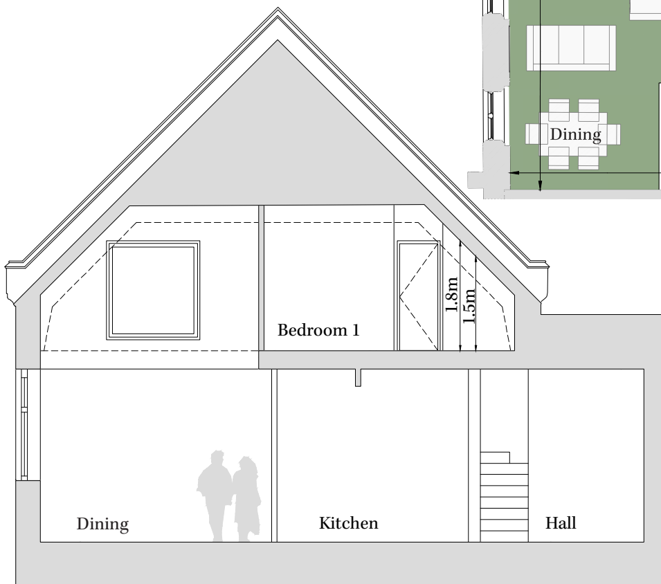
Section - NTS
