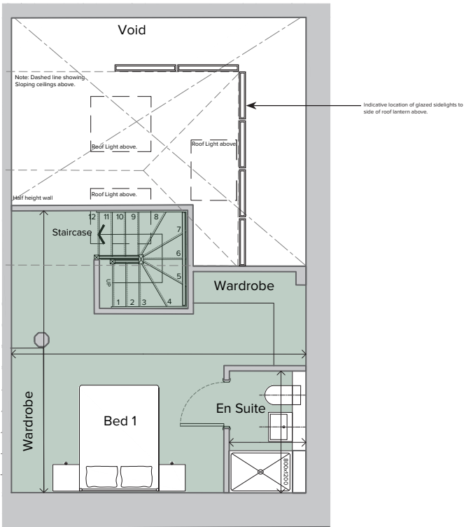
First Floor Mezzanine Plan
