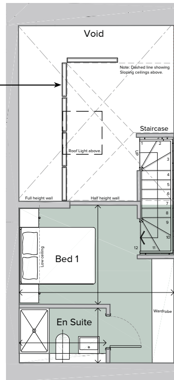
First Floor Mezzanine Plan
