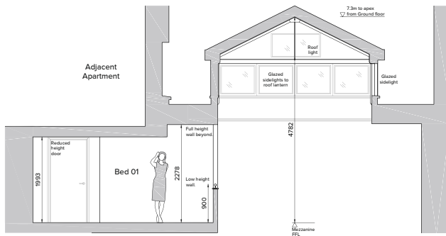
Section Through Mezzanine
