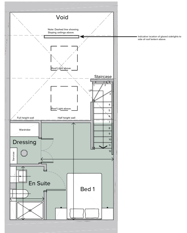
First Floor Mezzanine Plan
