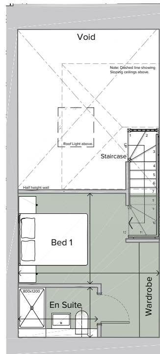
First Floor Mezzanine Plan
