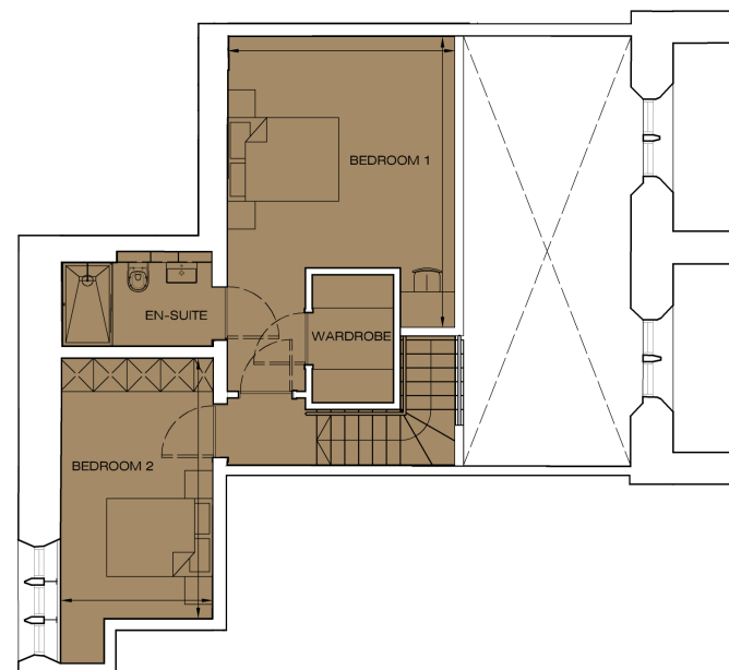
FLAT F29 - MEZZANINE FLOOR PLAN
